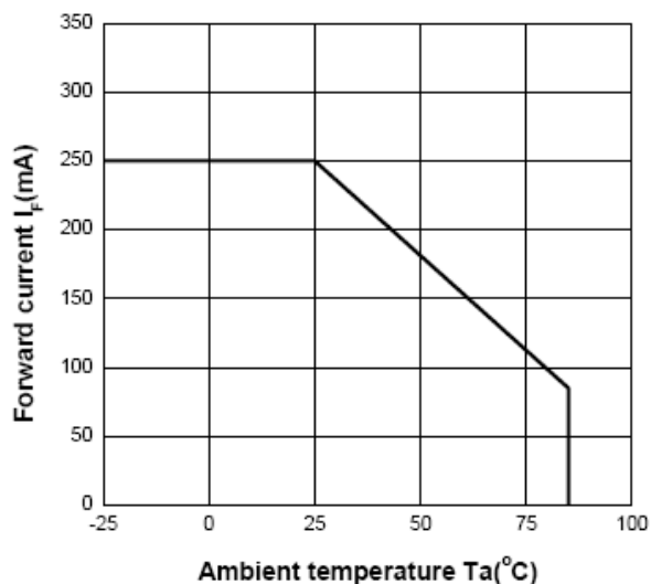
Forward Current Derate Curve
