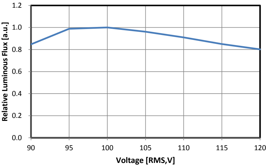
Fig 6. Relative Luminous Flux vs. Voltage, T_a=25^{\circ}\text{C} , 120V
